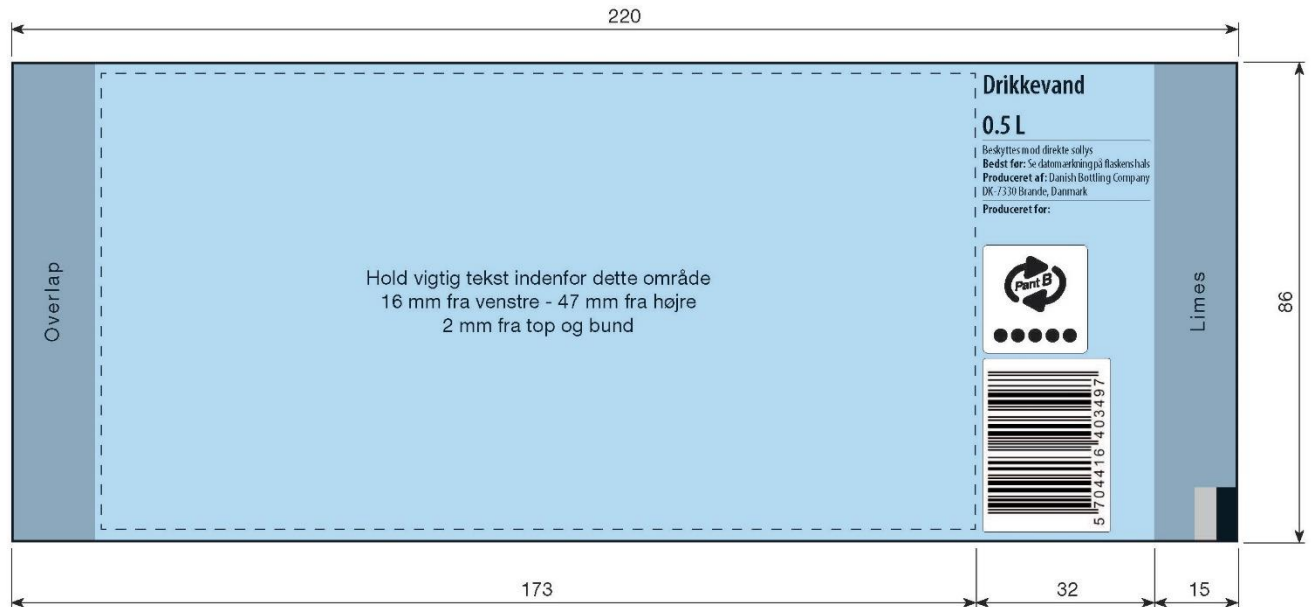
Figur: Plantegning over label – Choice 50 Plastic
